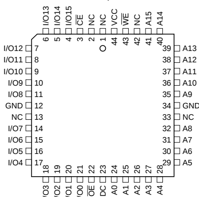
PLCC Top View
